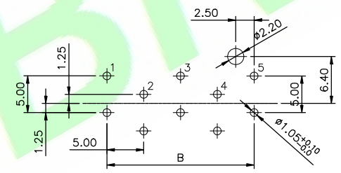
For Terminal Type 1 P.C.B Layout
