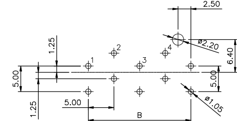
For Terminal Type 2 P.C.B Layout
