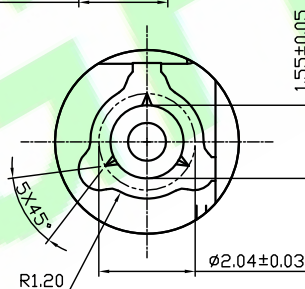
Detail C 3:1
