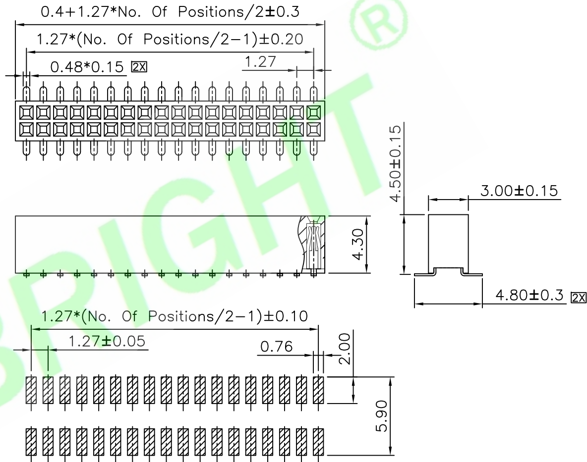
Recommended PCB Layout(Tolerance:0.05mm)
