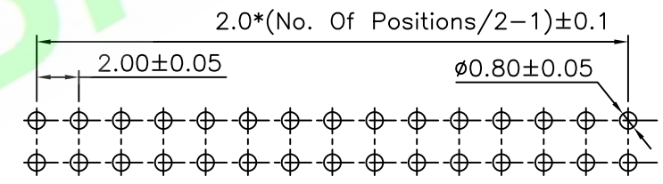
Recommended PCB Layout(Tolerance:0.05mm)
