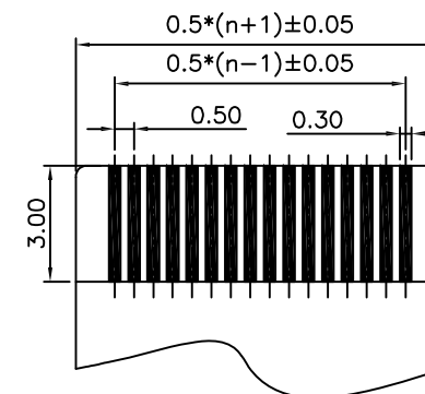
FFC/FPC Dimension(Thickness 0.30 mm)
