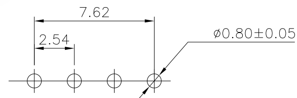
PCB LAYOUT
