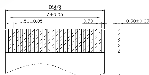
FFC/FPC Dimension
