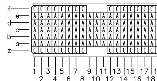
Contact Layout
