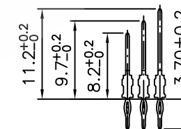
Pin Type
