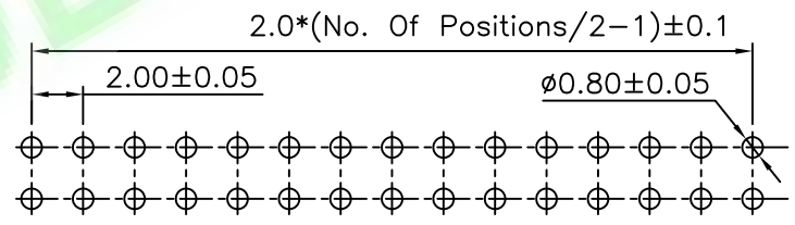
Recommended PCB Layout(Tolerance:0.05mm)
