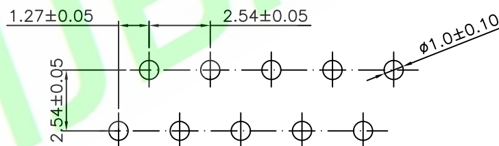
PCB LAYOUT
