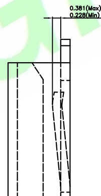
DETAIL "B"
