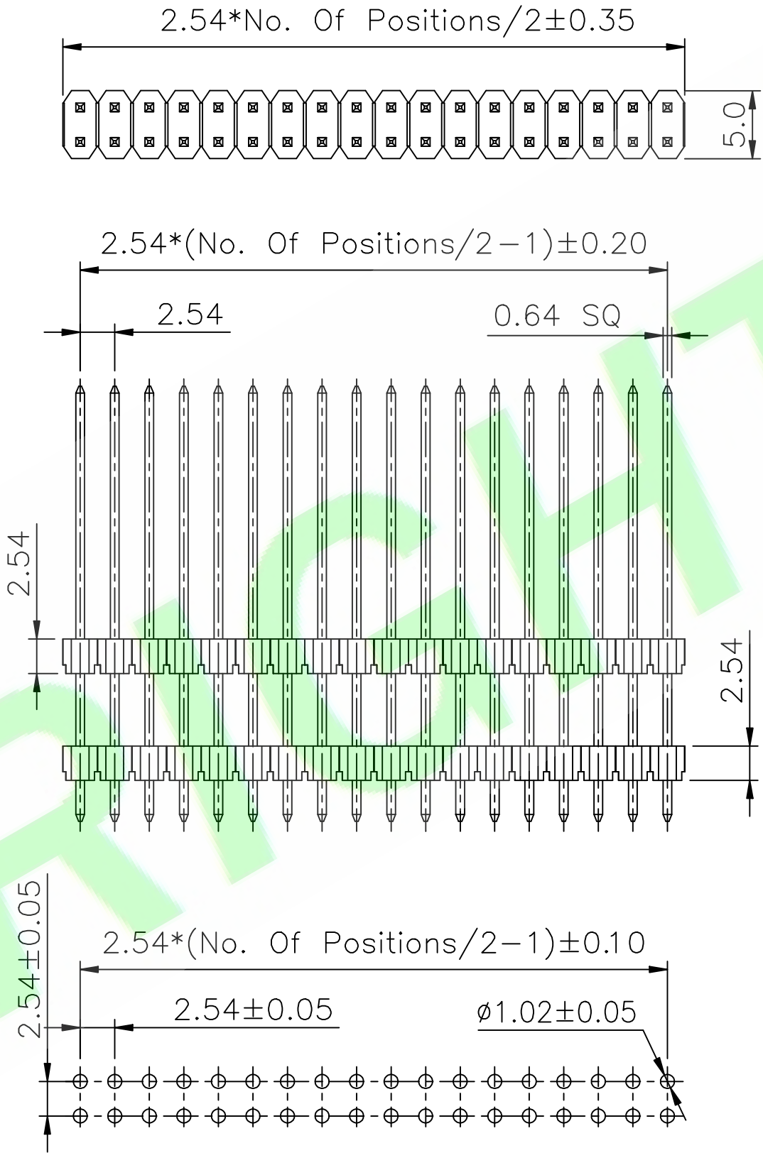
Recommended PCB Layout
