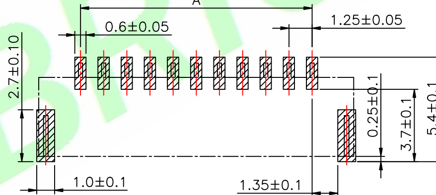
PCB LAYOUT
