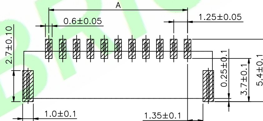
PCB LAYOUT
