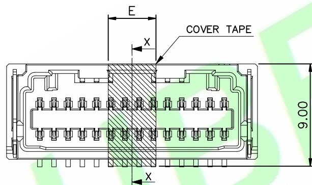
WITH COVER TAPE
