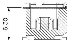
34-42 CIRCUIT
