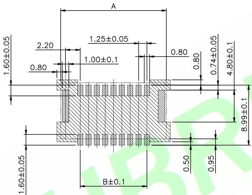
PCB LAYOUT
