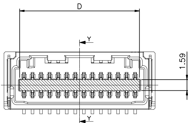
WITHOUT COVER TAPE
