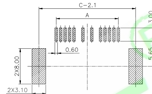
PCB LAYOUT (TOP VIEW) Tolerance:±0.05mm
