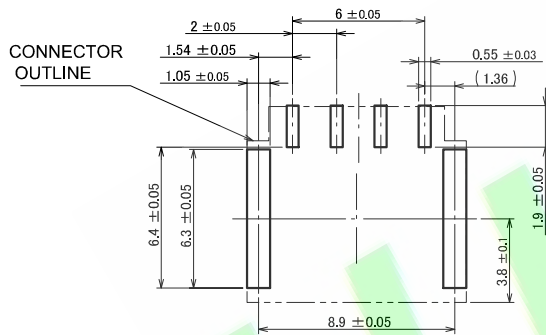
Recommended PCB LAYOUT (TOP VIEW) Tolerance: ±0.05mm
