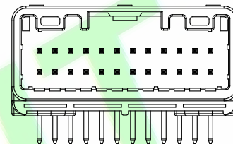
24 PIN
