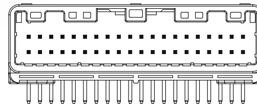
40 PIN
