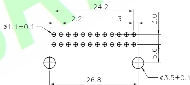
PCB LAYOUT GENERAL TOLERANCE:±0.05
