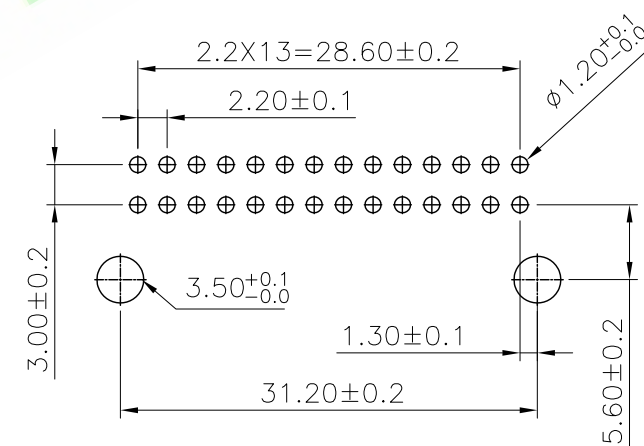
PCB LAYOUT
