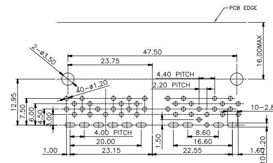
Recommended PCB LAYOUT (TOP VIEW) Tolerance: ±0.05mm
