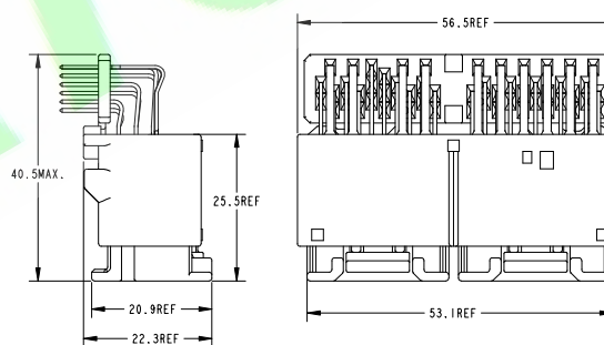
CAP ASSEMBLY AND PLUG ASSEMBLY ENGAGEMENT DRAWING
