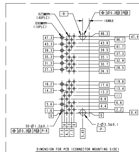
DIMENSION FOR PCB (CONNECTOR MOUNTING SIDE)
