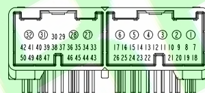
FIG. 1 CIRCUIT NUMBERS
