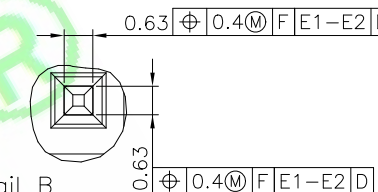
Detail B Scale 10:1 8 Places
