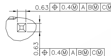
Detail A Scale 10:1 8 Places
