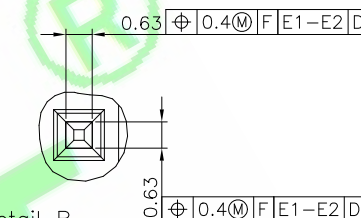
Detail B Scale 10:1 16 Places
