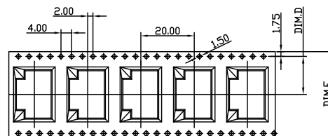
05~11 CONTACTS PULL OUT DIRECTION 产品引出方向
