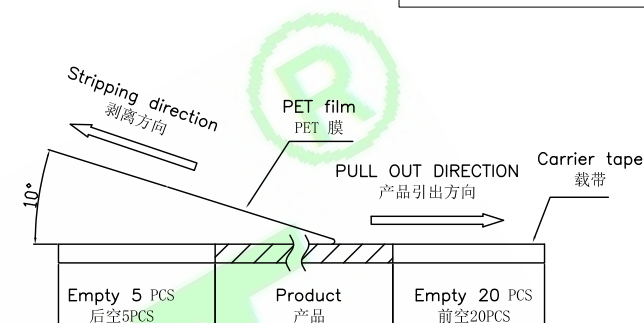
Schematic diagram of PET film peeling PET膜剥离示意图
