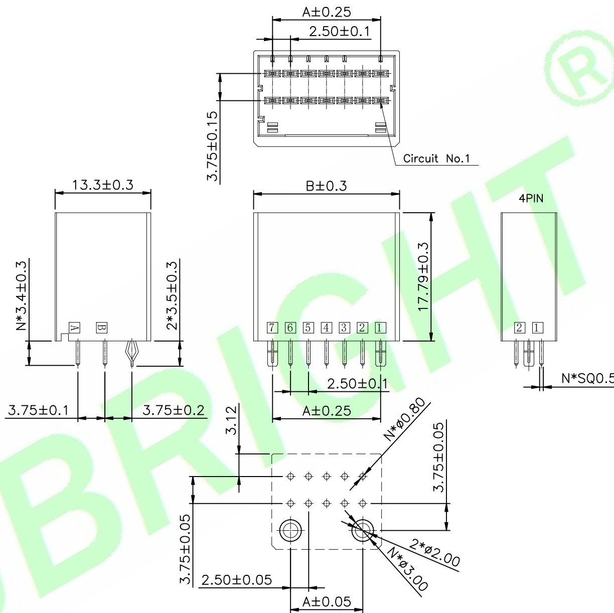
Recommended PCB LAYOUT
