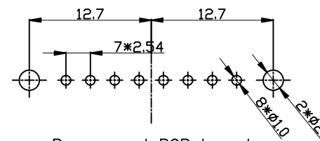
Recommend PCB Layout
