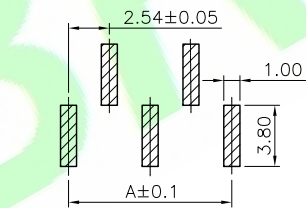
A Type Recommended PCB Layout
