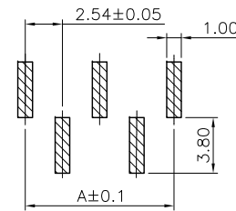
B Type Recommended PCB Layout
