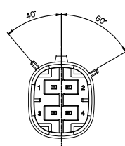
B Type Light Gray
