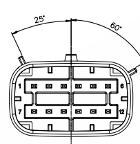
B Type Light Gray
