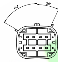
C Type Drak Gray
