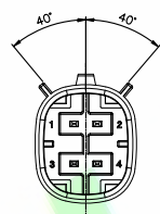
D Type Black 4P
