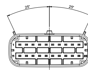
D Type Black or Light Gray 20P
