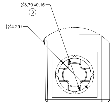
DETAIL A SCALE 10:1
