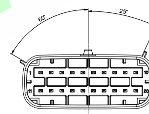
C Type Brown
