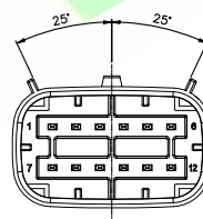
D Type Black 12P
