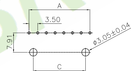
PCB Layout (4~12P)
