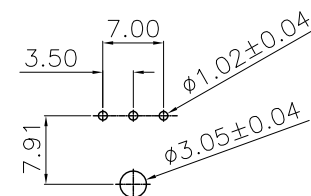
PCB Layout (2~3P)
