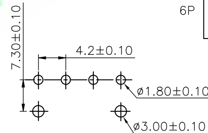
3P-6P PCB Layout
