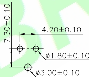
2P PCB Layout
