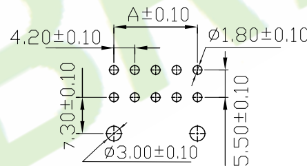
P.C.B LAYOUT: Component Side 3P-12P Recommended PCB Thickness 1.78MAX
