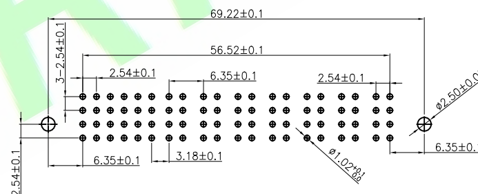
PCB LAYOUT
