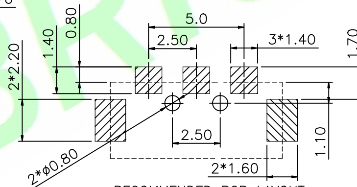
RECOMMENDED PCB LAYOUT TOP VIEW(±0.05)
