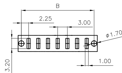
P.C. Board Hole Pattern
