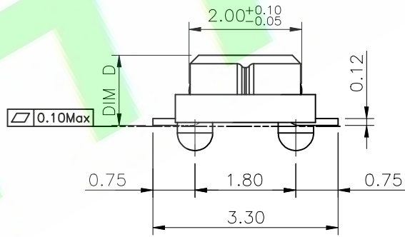
Assembly Female: BM0500M-XXAF-XX-XG
