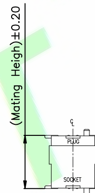
Mating Height
