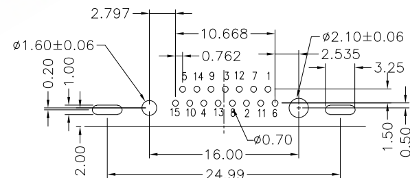
PCB LAYOUT
