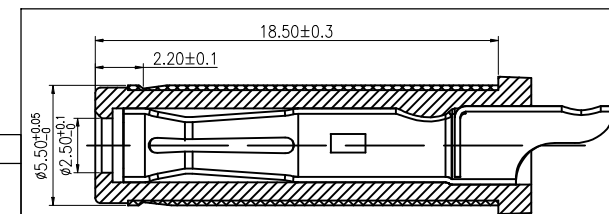
MATING PLUG P/N: DP5525-0063-00
