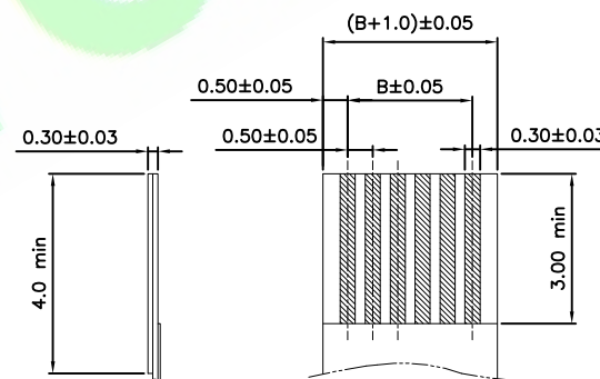
FFC/FPC Dimension(Thickness 0.20 mm)
