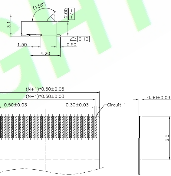
RECOMMENDED FPC/FFC DIMENSION
