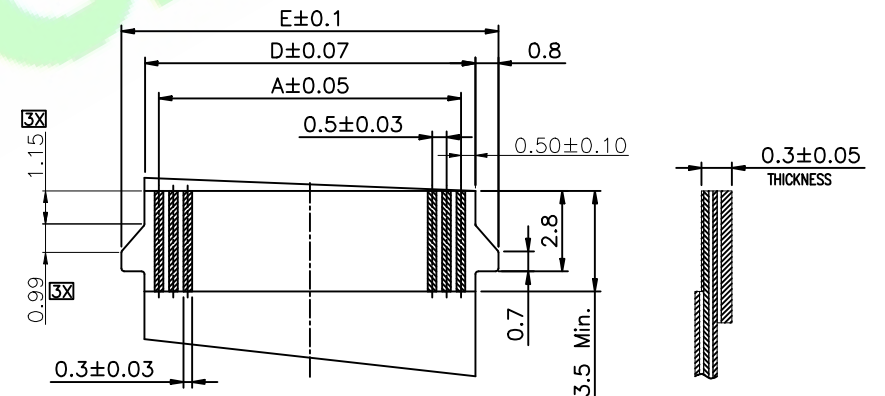
Accommodated FFC/FPC
