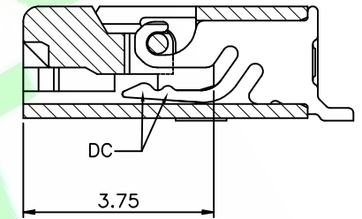
Double Contact SCALE 2:1
