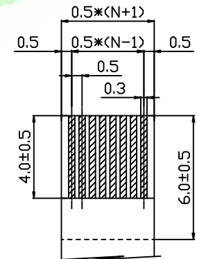
APPLICABLE FPC OF GOLD PLATING RECOMMENDED DIMENSION
