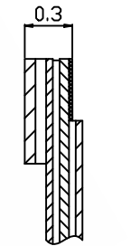
STRUCTURE OF FPC
