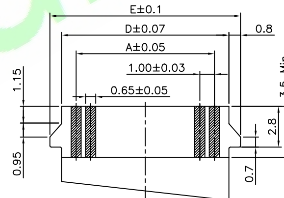
Accommodated FFC/FPC
