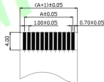
FFC/FPC Dimension(Thickness 0.30mm)
