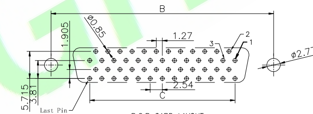
P.C.B. BOARD LAYOUT (50Pin) R1 Type/ reverse side foot position
