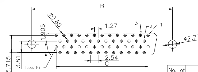
P.C.B. BOARD LAYOUT (50Pin) R2 Type/ reverse side foot position
