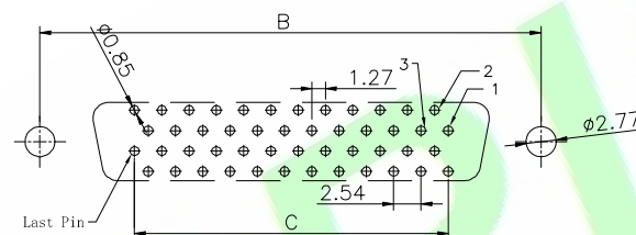
P.C.B. BOARD LAYOUT (68100Pin) R1 Type/ reverse side foot position
