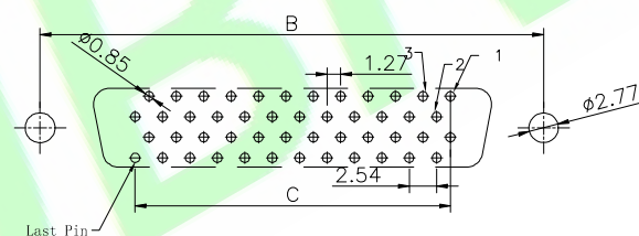
P.C.B. BOARD LAYOUT (68100Pin) R2 Type/ reverse side foot position
