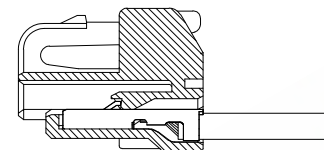
TERMINAL ASSEMBLY DRAWING
