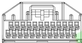
24P A TYPE
