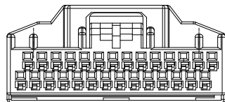
28P A TYPE
