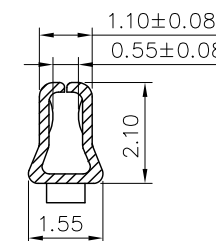
SEC: C-C
