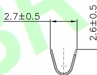
SECT. A-A
