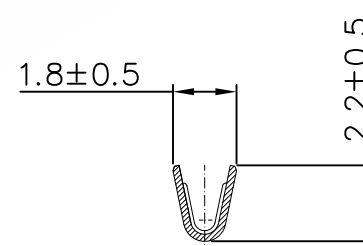
SECT. B-B
